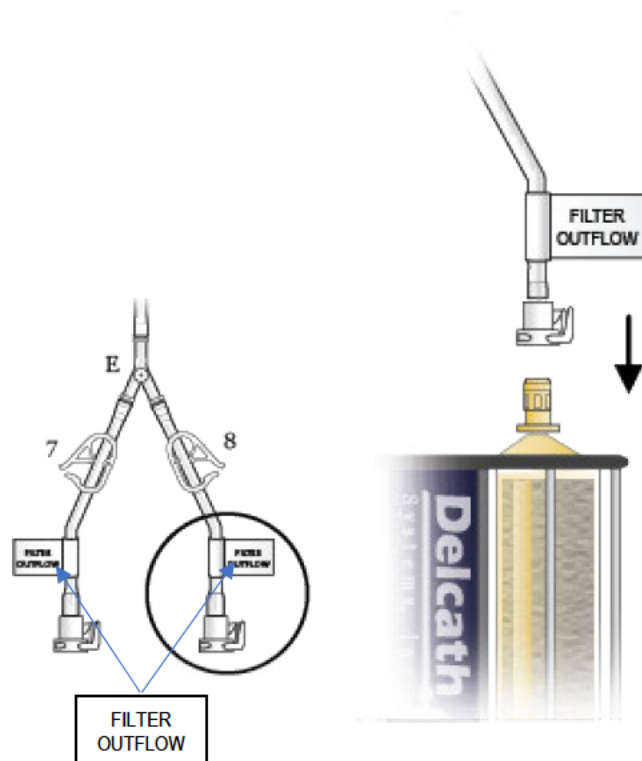
Figure 8: Filter Outflow Line Connection
