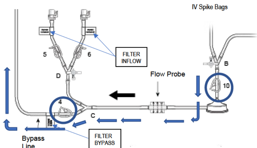
Figure 15: Priming Bypass Line
