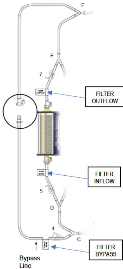
Figure 9: Bypass Line Assembly
