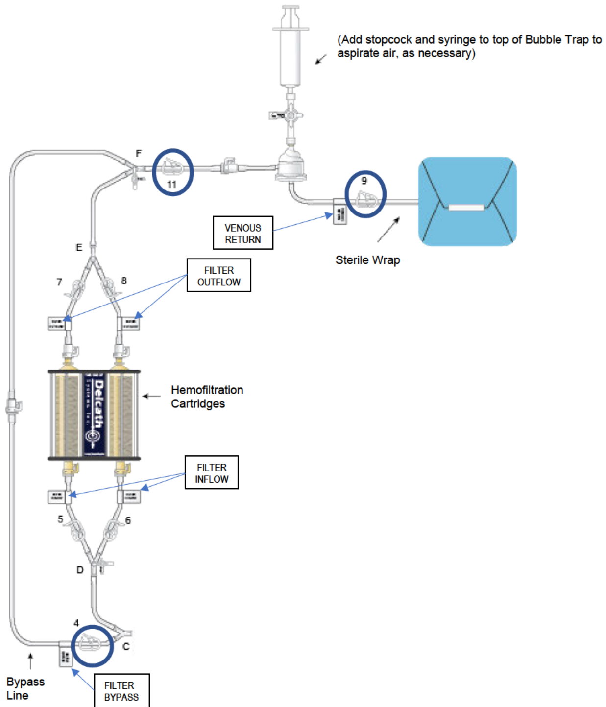
Figure 19: Priming Venous Return Line with Built-In Bubble Trap
