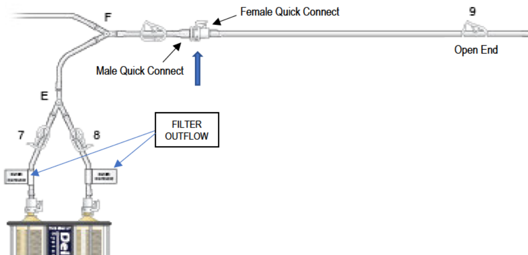
Figure 10: Prime Flush Line Assembly Connection
