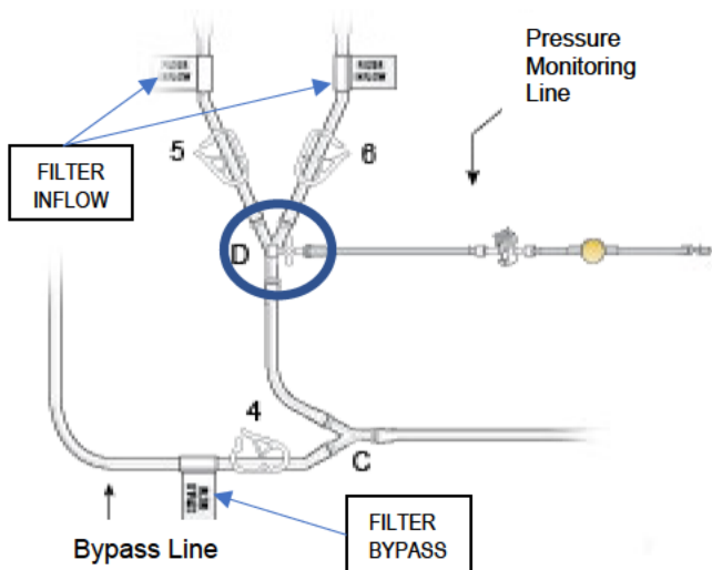
Figure 21: Attach and Prime Pre-Filter (Post-Pump) Pressure Line
