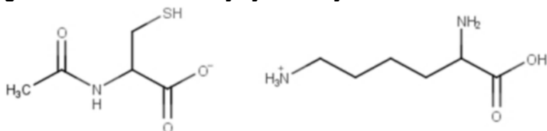
Figure 3. Structure of Acetylcysteine Lysine
