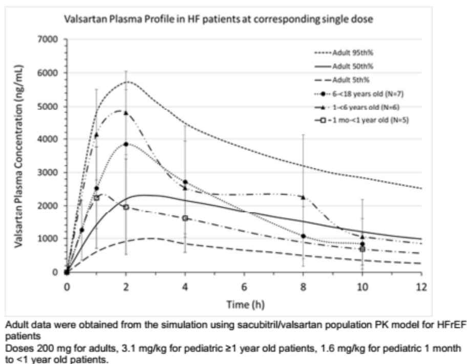
Figure 4.3.3.3 Plasma concentration vs. time profiles for valsartan among adult and pediatric patients at corresponding sacubitril/valsartan single dose ( Source: Figure 11-7 of Study CLCZ696B2319 CSR Ver. 2, NDA 207620, eCTD 0188, M 5.3.5.1)
