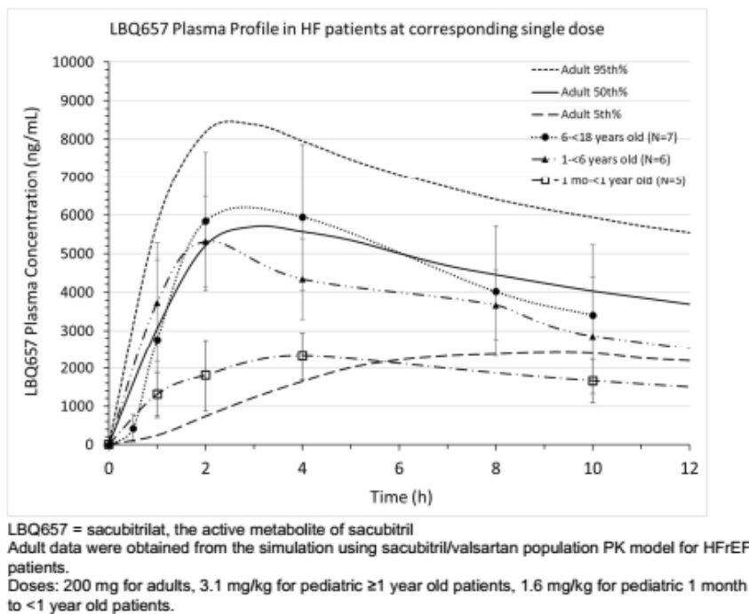
Figure 4.3.3.2 Plasma concentration vs. time profiles for sacubitrilat (Active metabolite) among adult and pediatric patients at corresponding sacubitril/valsartan single dose ( Source: Figure 11-7 of Study CLCZ696B2319 CSR Ver. 2, NDA 207620, eCTD 0188, M 5.3.5.1)
