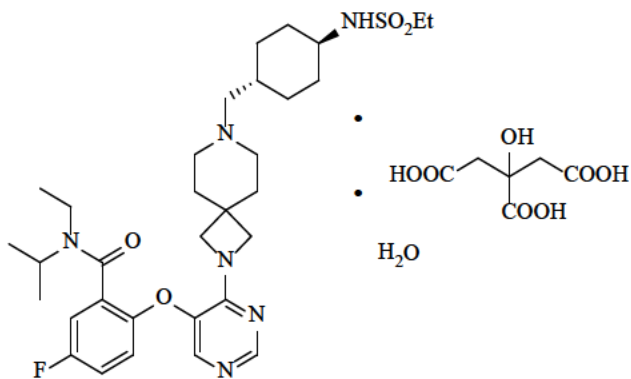
Figure 1: Chemical structure of Revumenib Citrate hydrate
