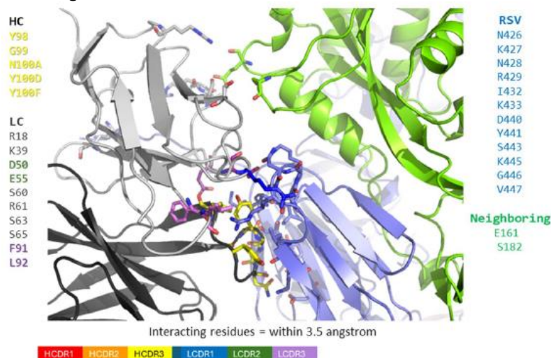
Figure 28. Crystal Structure of the Clesrovimab Parent RB-1 Fab and RSV Prefusion F Complex Showing the Interaction Points Between RB-1 and F Protein
