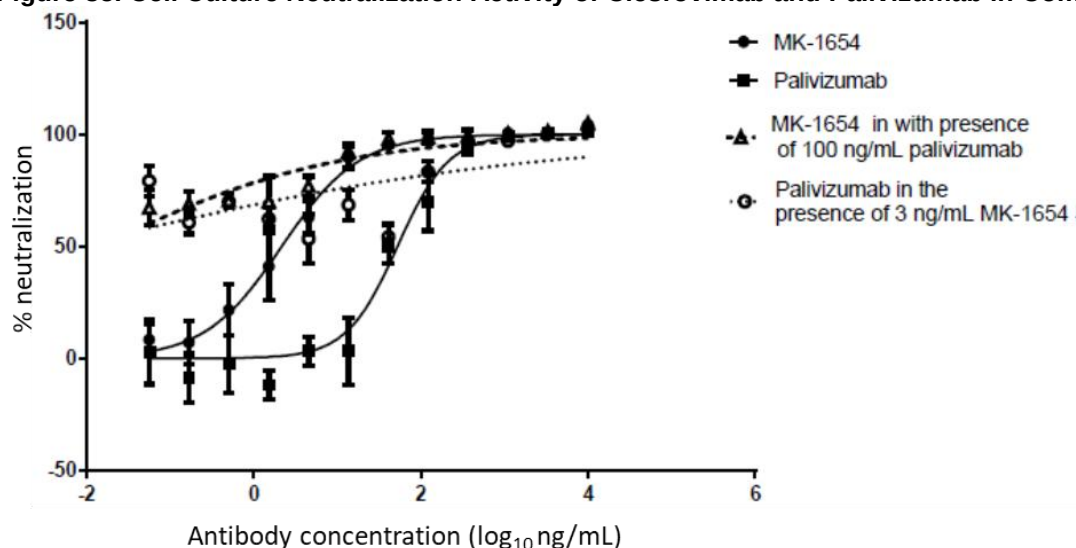
Figure 35. Cell Culture Neutralization Activity of Clesrovimab and Palivizumab in Combination
