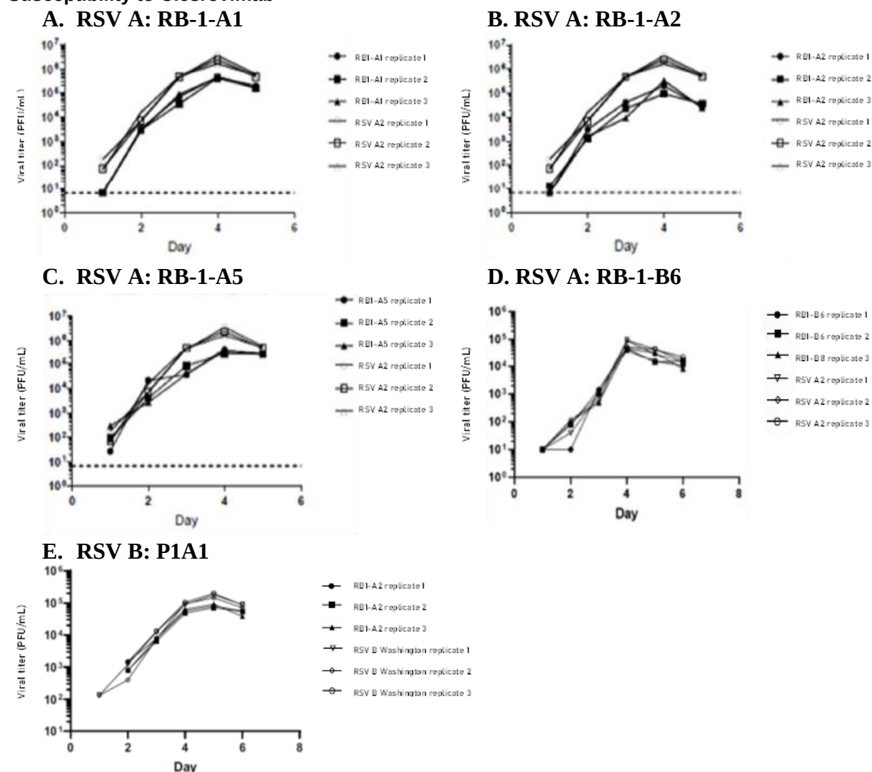
Figure 36. Replication Dynamics of Cell Culture Selected RSV Variants With Reduced Susceptibility to Clesrovimab
