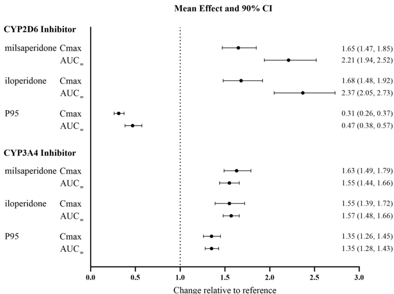
Figure 1: Effect of CYP3A4 and CYP2D6 Inhibitors on the Pharmacokinetics of Milsaperidone, Iloperidone, and P95
