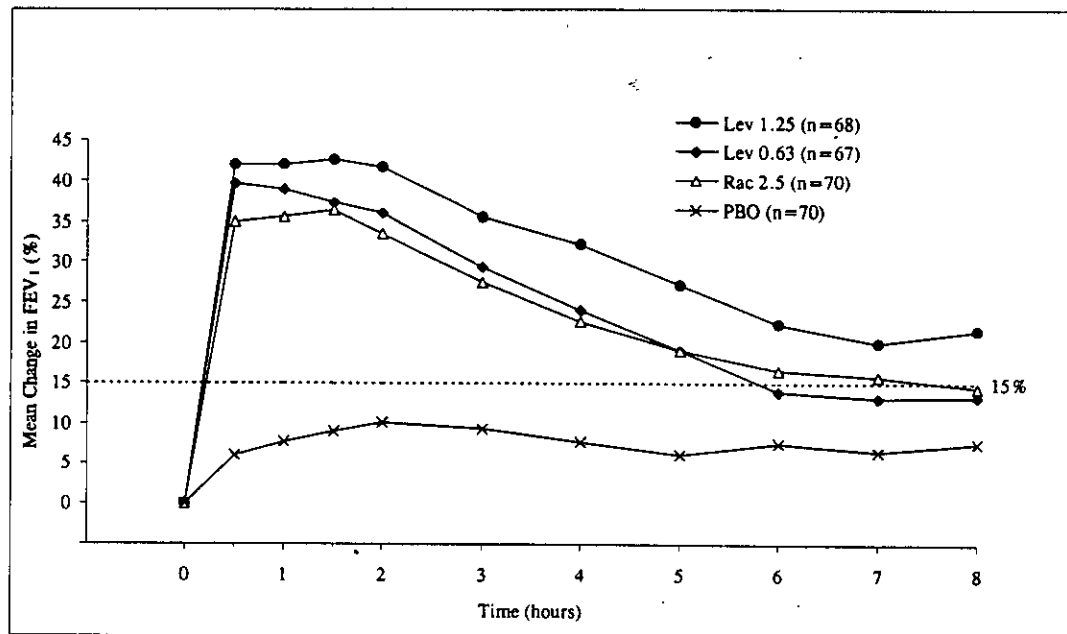
Figure 1: Mean Percent Change from Baseline in FEV 1 on Day 1, All Patients
